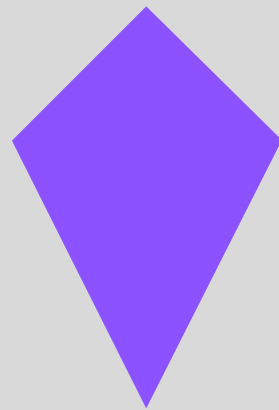
Kite
