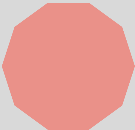
Decagon
