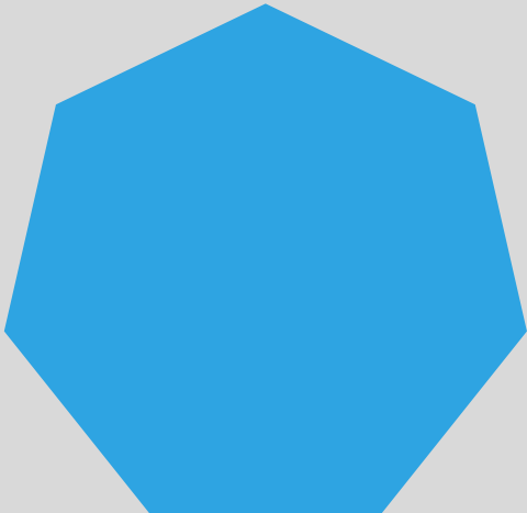
Heptagon
